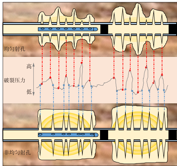
图2 射孔簇点位置优化调控裂缝均衡延伸示意图 Fig. 2 Schematic diagram of perforation cluster position optimization to control uniform propagation of fractures
